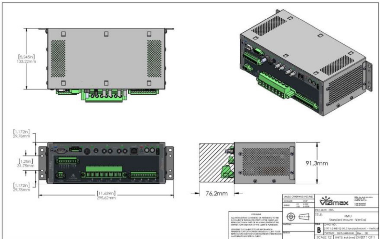
Figure 7 PMU standard configuration – Vertical
