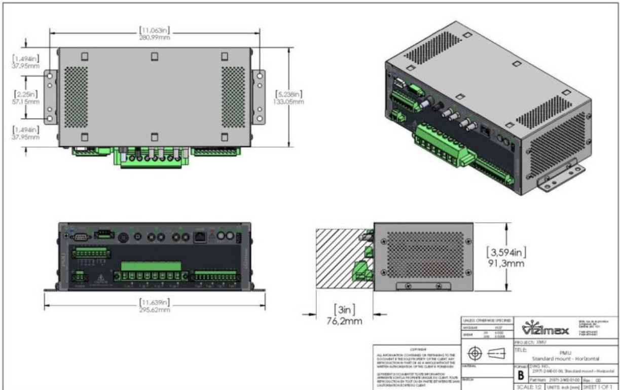
Figure 6 PMU standard configuration standard – Horizontal
