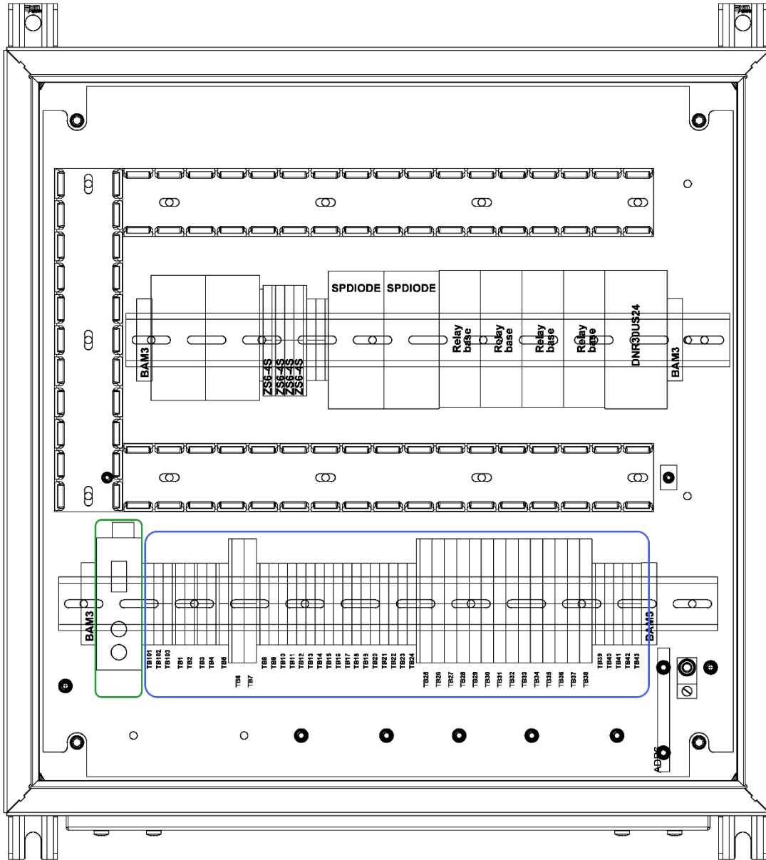
FIGURE 3 TERMINAL BLOCKS LOCATION IN STM045000 ENCLOSURE
