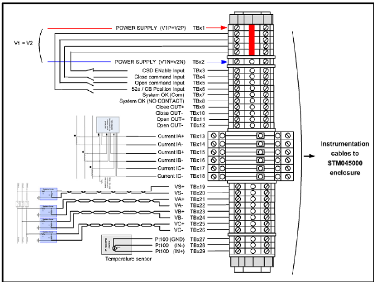
FIGURE 5 EXAMPLE OF SUGGESTED TERMINAL BLOCKS INSTALLED IN MV SWITCHGEAR
