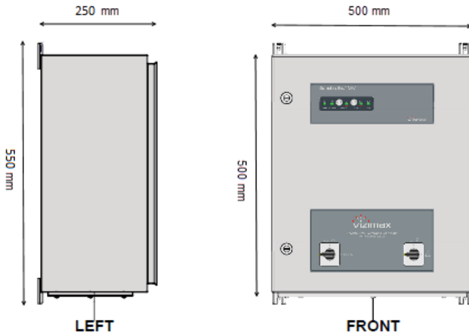
FIGURE 6 STM045000 MOUNTING POINTS AND EXTERNAL DIMENSIONS
