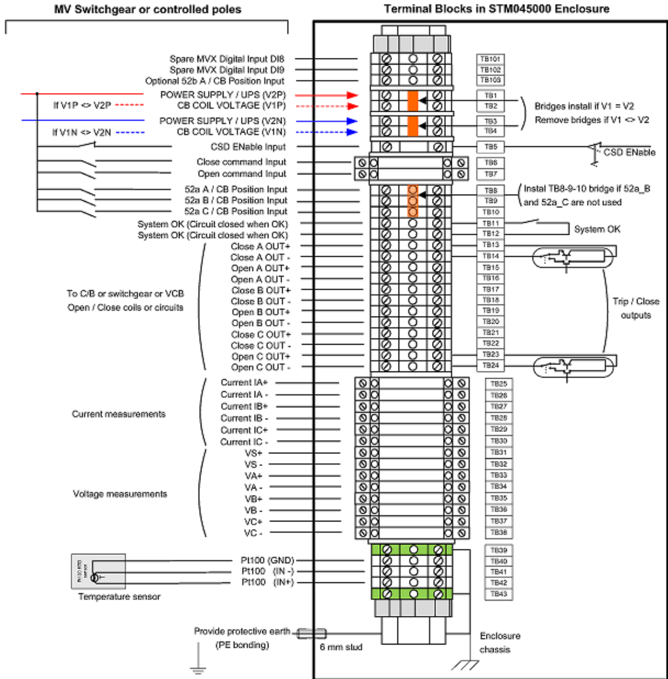
FIGURE 4 STM045000 TERMINAL BLOCKS IDENTIFICATION
