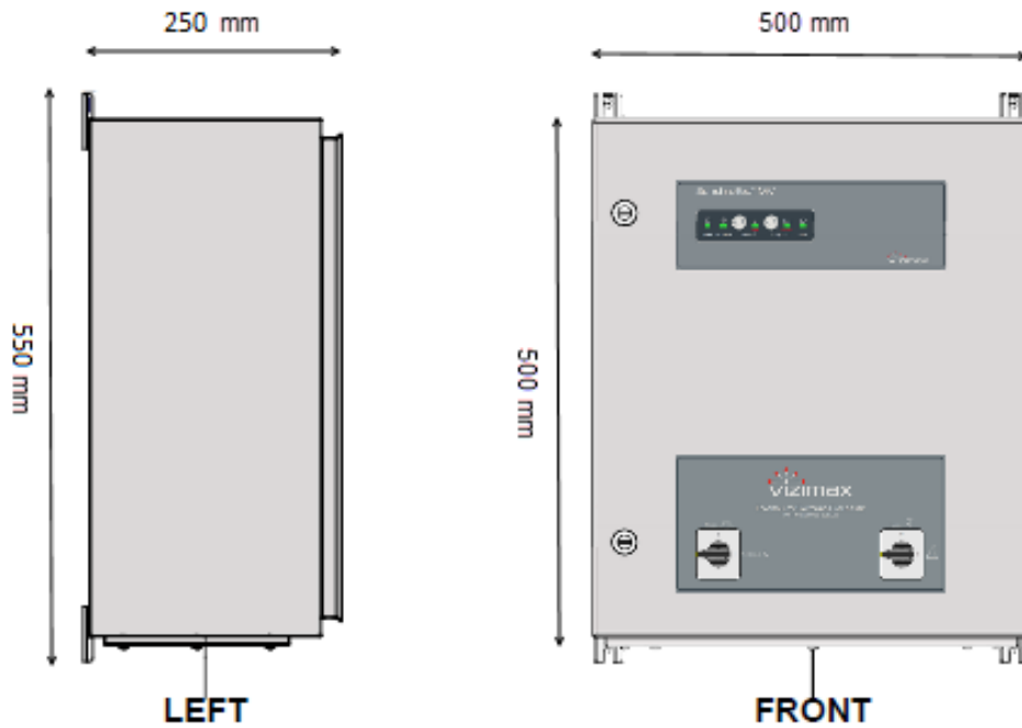
FIGURE 6 STM045000 MOUNTING POINTS AND EXTERNAL DIMENSIONS
