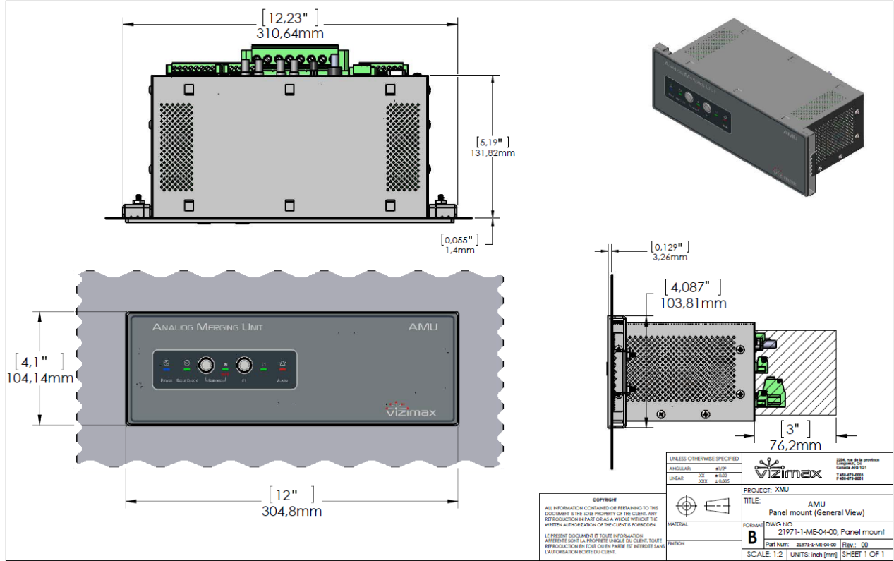
FIGURE 8 PANEL MOUNT CONFIGURATION
