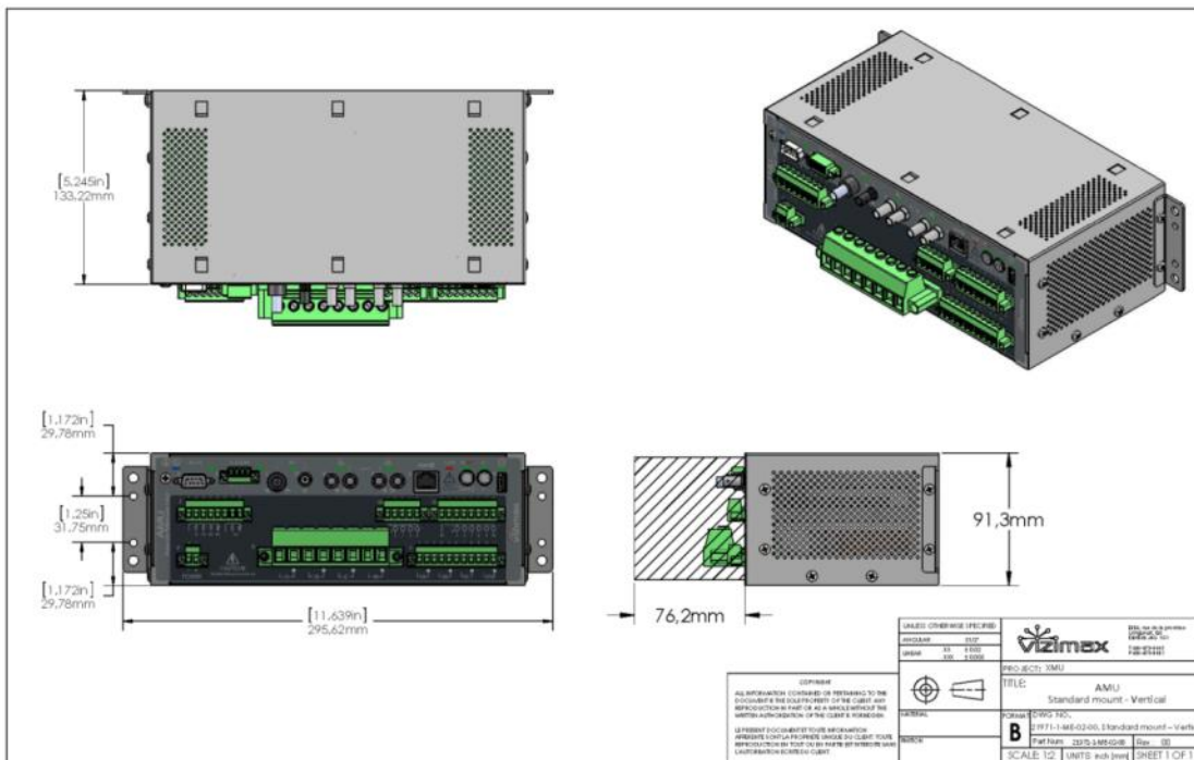
FIGURE 7 STANDARD CONFIGURATION —VERTICAL
