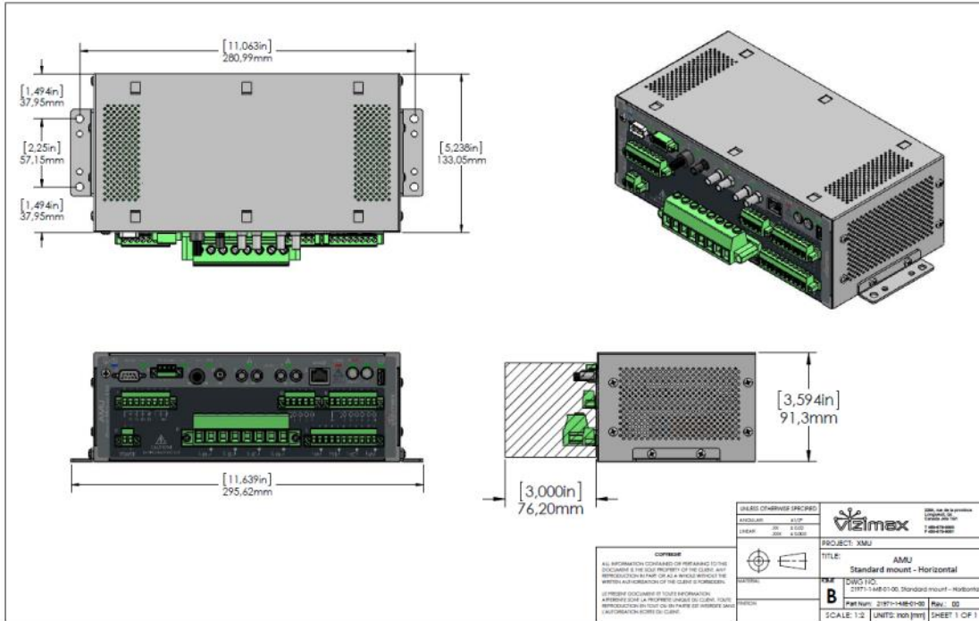
FIGURE 6 STANDARD CONFIGURATION —HORIZONTAL
