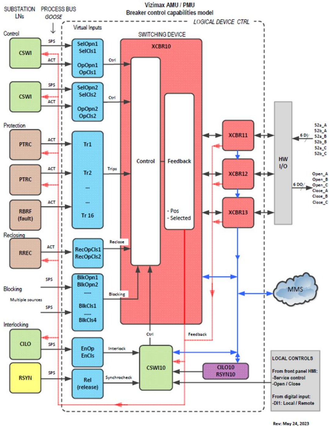
FIGURE 3 PMU 61850 GOOSE SUBSCRIBER XCBR CAPABILITIES MODEL
