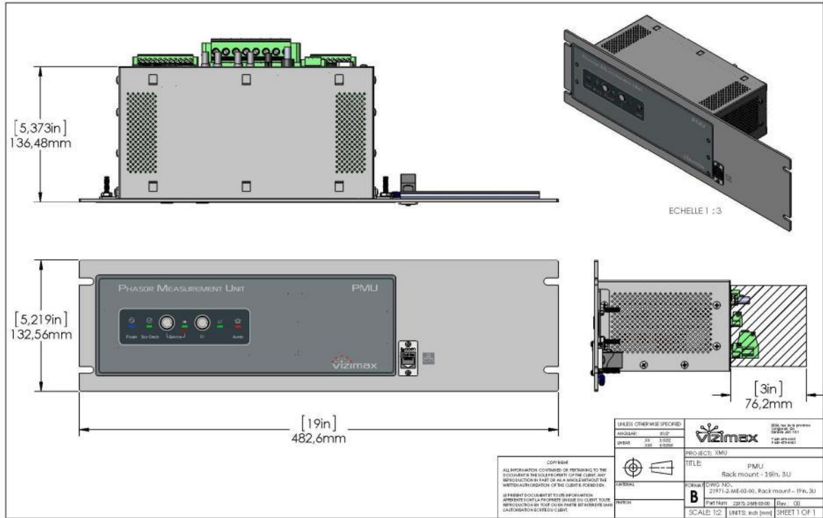
FIGURE 8 19" RACK MOUNT CONFIGURATION
